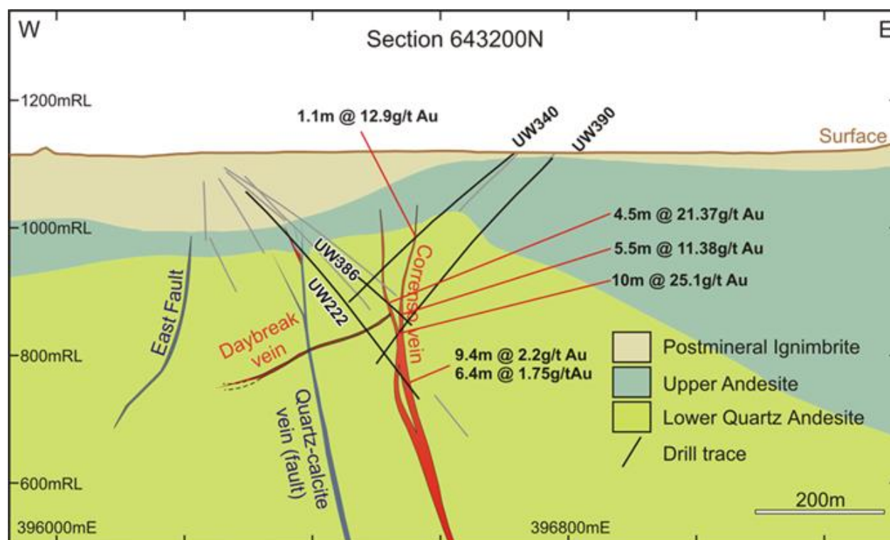
Figure 6: Geological Section, Correnso Project (643200mN)
